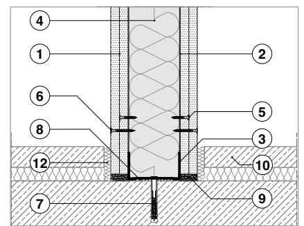
Fig. 17. Connecting a partition wall with concrete floor and dry screed panels with dry jointless floor against the wall
