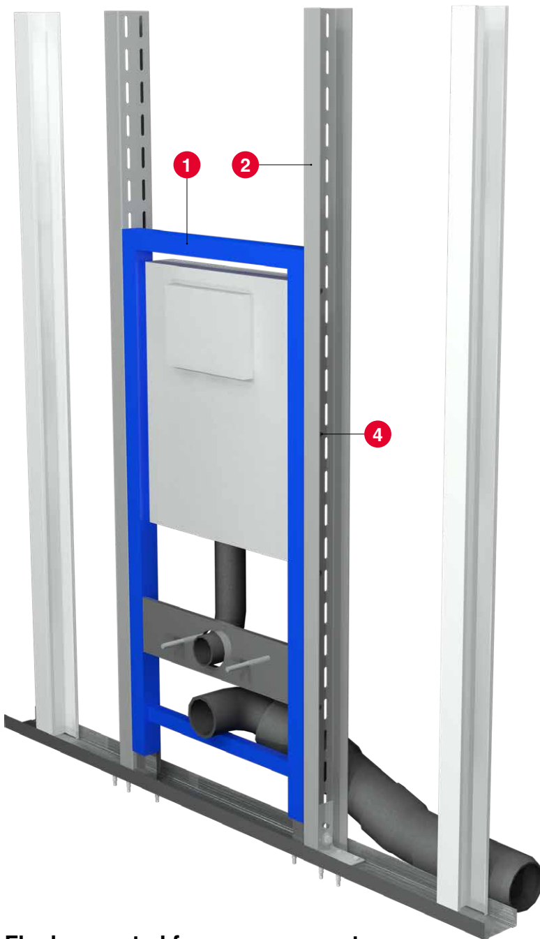
Sanitary flush-mounted frame in a partition wall
