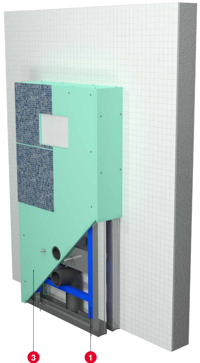
Sanitary flush-mounted frame installation
