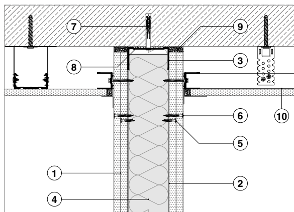
Fig. 5. Connecting a partition wall with NORGIPS ceiling lining
