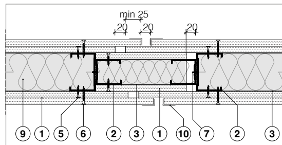
Fig. 29. Expansion joint – variant 4
