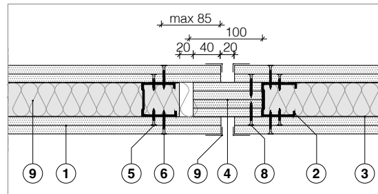
Fig. 27. Expansion joint – variant 2
