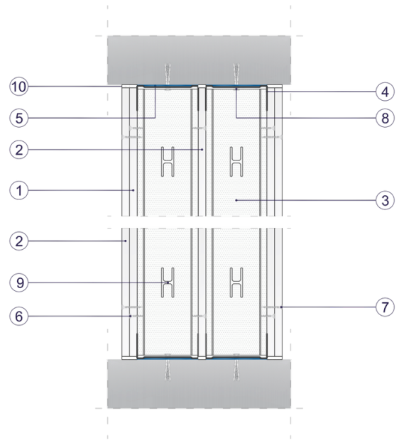
Fig. 3. Partition wall vertical section
