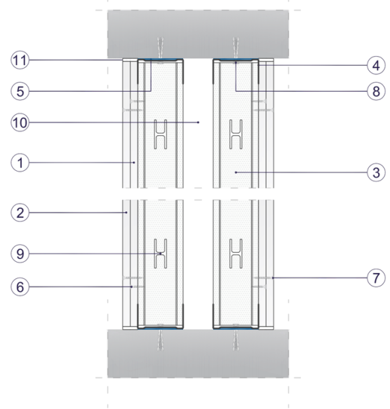
Fig. 3. Partition wall vertical section
