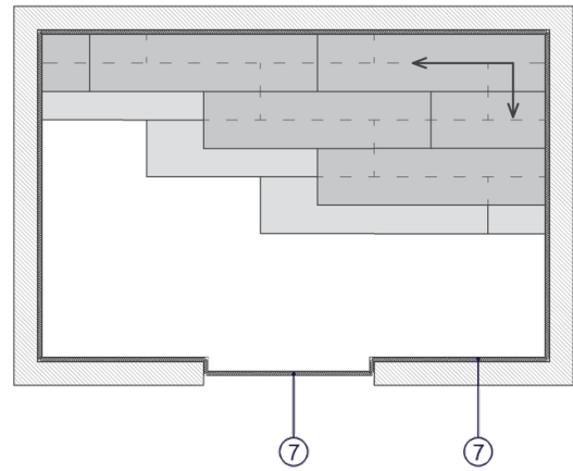
Fig. 3. Board laying sequence
