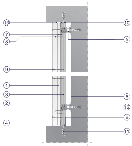
Fig. 3. Wall cladding vertical section
